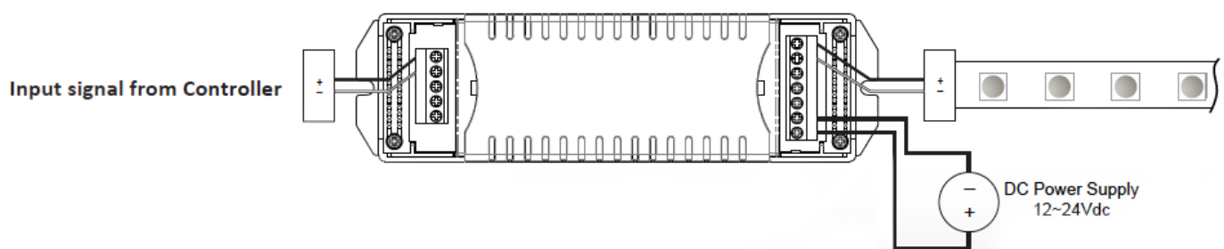
SHWC and Repeater Wiring
